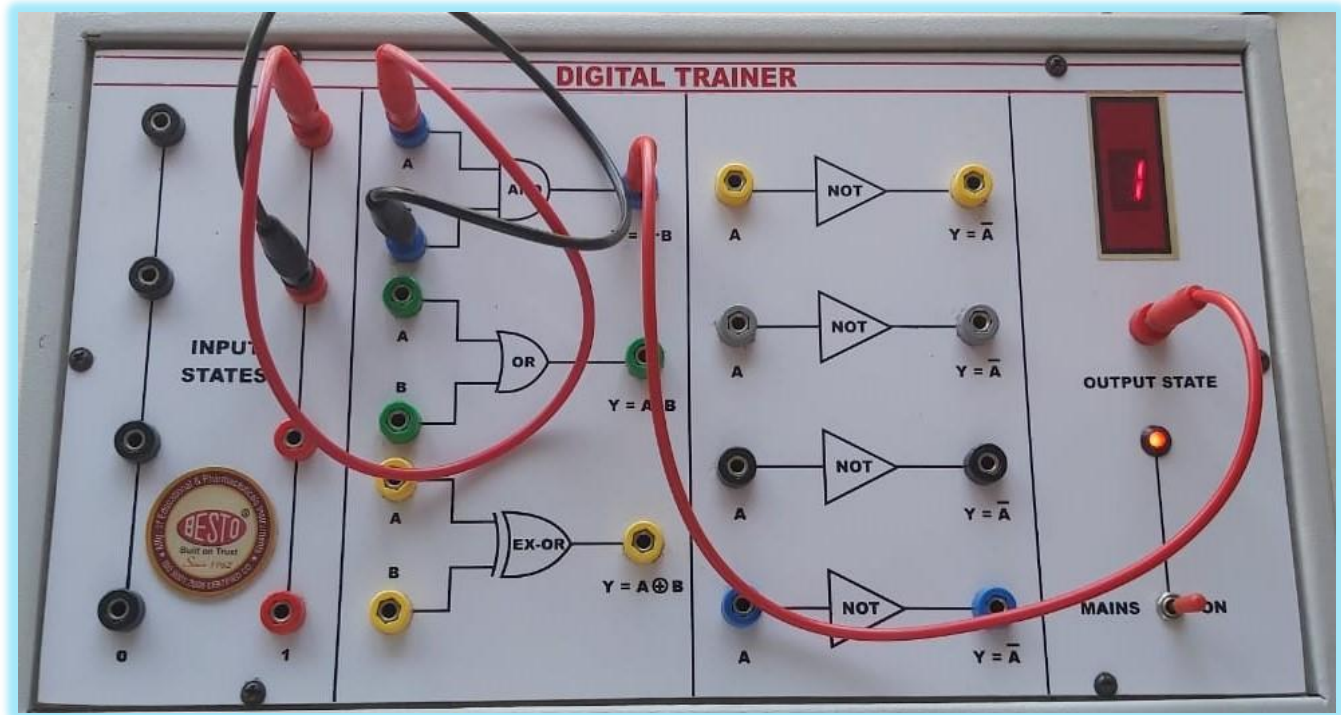
LOGIC GATE CIRCUIT
