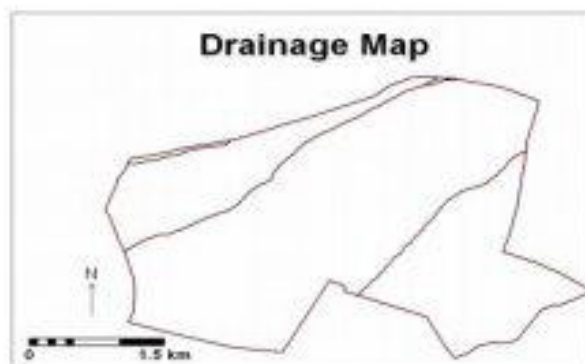
Map No. 2: Drainage Map
